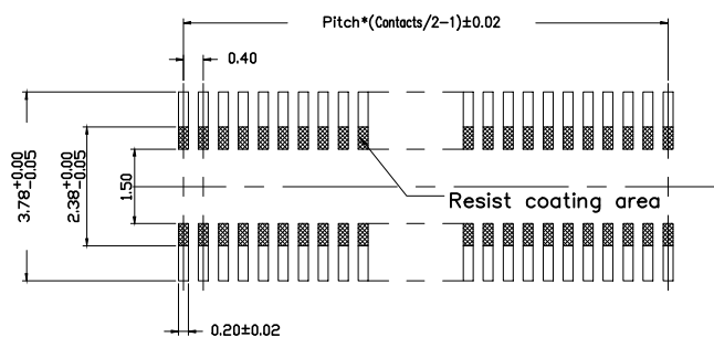
RECOMMENED P.C.B LAYOUT
