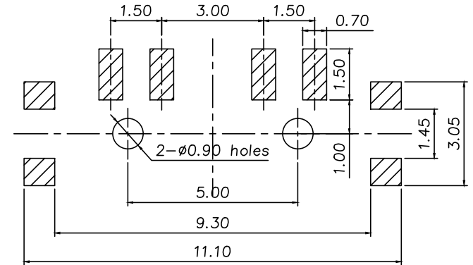
P.C.B Mounting Pattern Dimension
