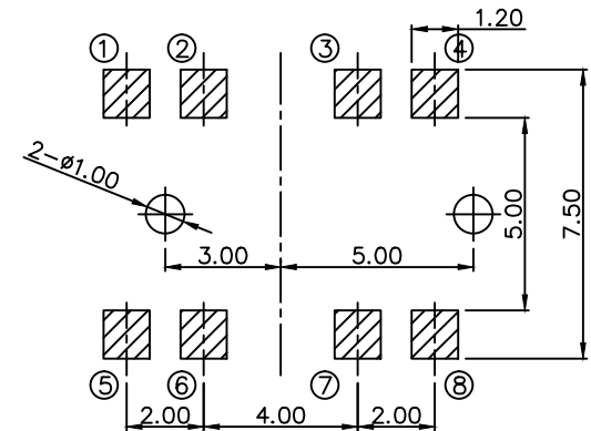
RECOMMENED P.C.B MOUNTING PATTERN DIMENSION
