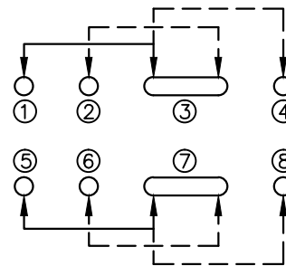
CIRCUIT DIAGRAM
