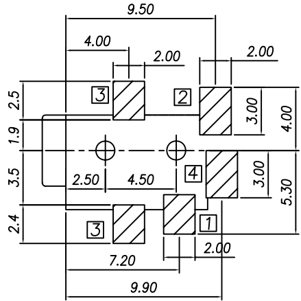
RECOMMENDED P.C.B. LAYOUT UNSPECIFIED TOLERANCE: ±0.1 (Top View)
