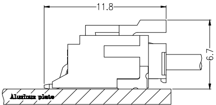
Assembly Layout
