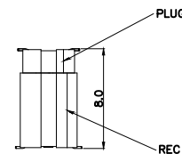
MATED HEIGHT
