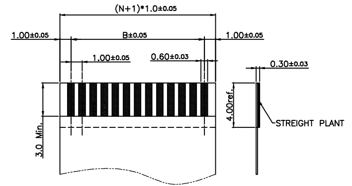
RECOMMENED FFC/FPC
