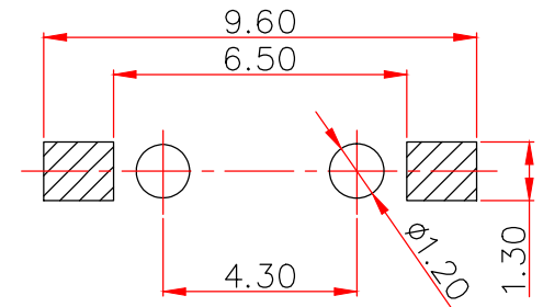
RECOMMENED P.C.B MOUNTING PATTERN DIMENSION
