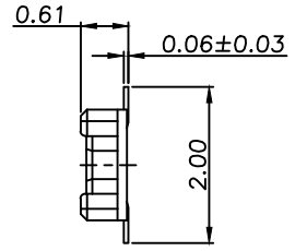
Matting drawing
