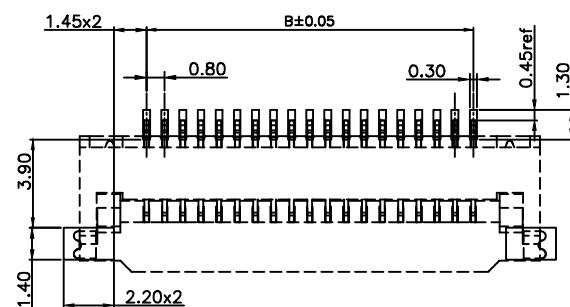
RECOMMENED P.C.B LAYOUT
