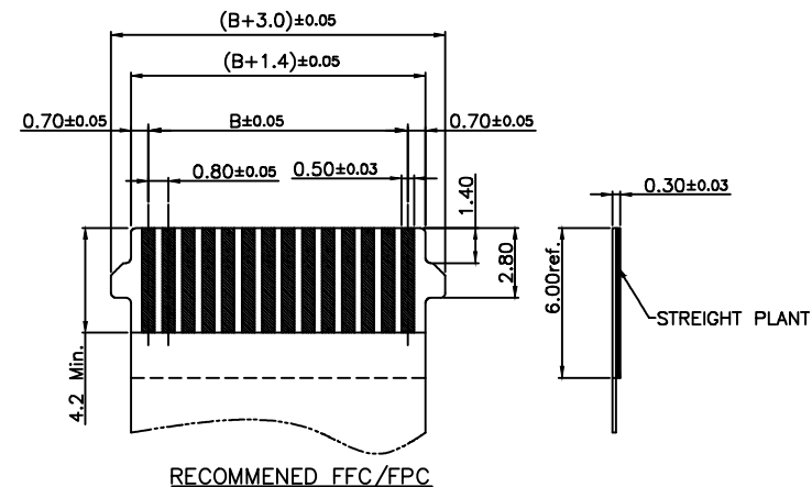
RECOMMENED FFC/FPC
