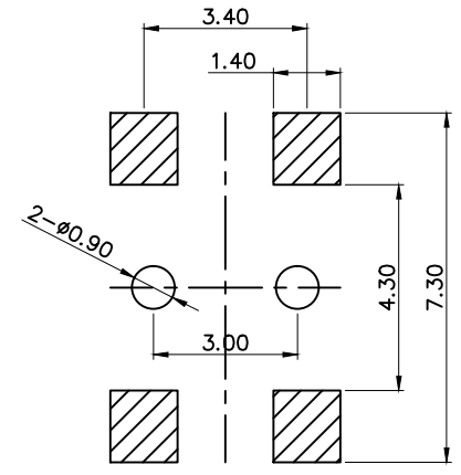
RECOMMENED P.C.B MOUNTING PATTERN DIMENSION
