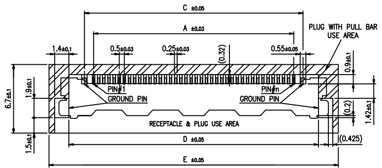
RECOMMENED P.C.B LAYOUT
