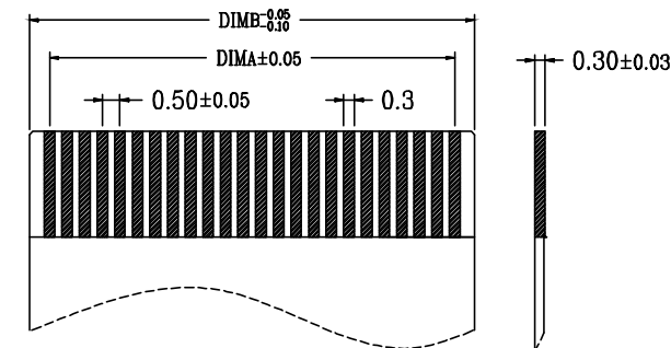
Applicable Flat Cable
