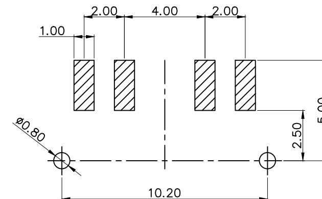
RECOMMENED P.C.B MOUNTING PATTERN DIMENSION
