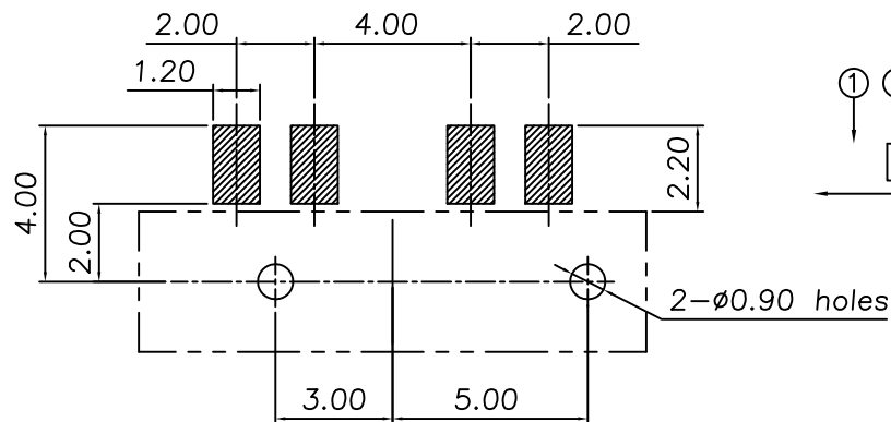
P.C.B Mounting pattern Dimension
