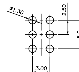
RECOMMENED P.C.B MOUNTING PATTERN DIMENSION
