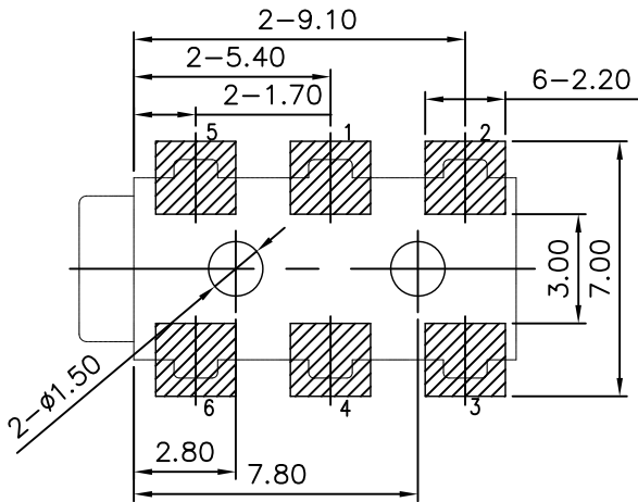
RECOMMENDED P.C.B MOUNTING PATTERN DIMENSION
