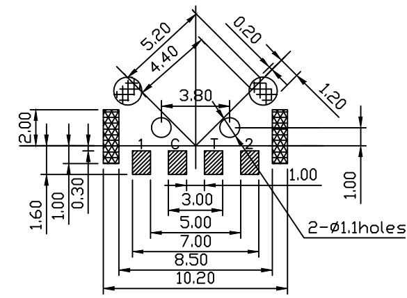
RECOMMENDED P.C.B MOUNTING PATTERN DIMENSION
