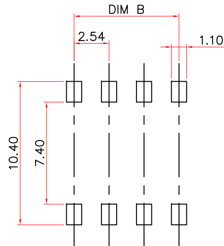
RECOMMENED P.C.B MOUNTING PATTERN DIMENSION
